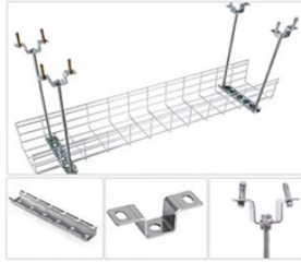
Ceiling installation
