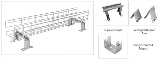
Lower Support Installation
